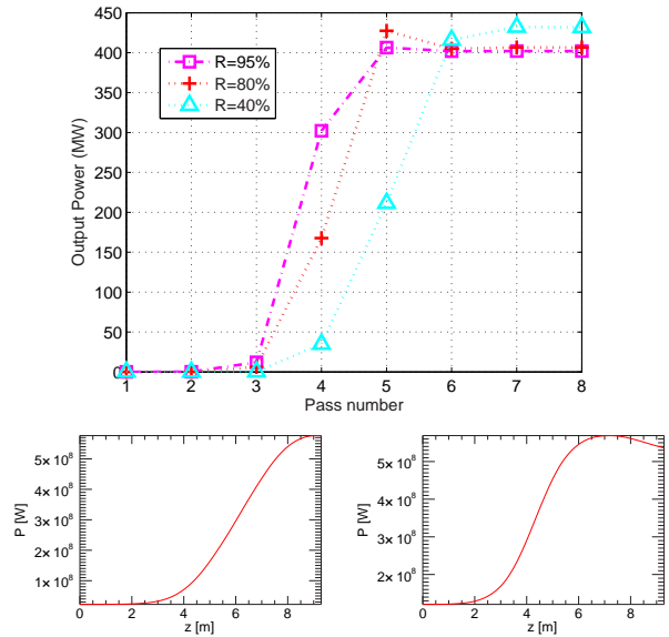
Figure 5: Top: pass to pass evolution from steady state Genesis 1.3 simulations. Lower left: evolution of intracavity intensity during pass 7 for 40% reflectivity mirrors. Lower right: evolution of intracavity intensity during pass 7 for 95% reflectivity mirrors.
