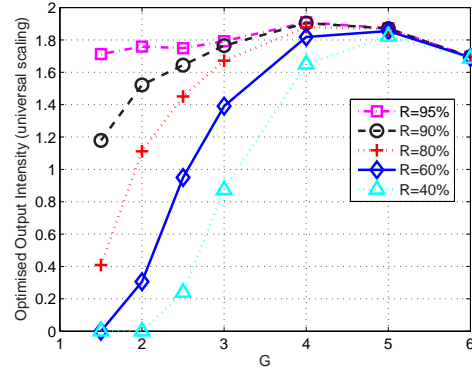
Figure 3: The optimised output intensity as a function of gain parameter G for a range of mirror reflectivities.
