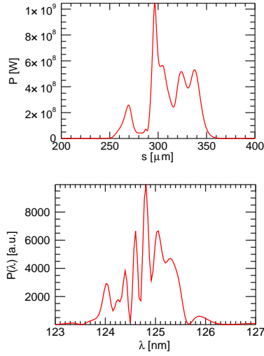
Figure 1: Genesis 1.3 simulation results showing SASE pulse profile and spectrum at saturation for 10eV photons. The estimated bandwidth is 0.8% (FWHM).
