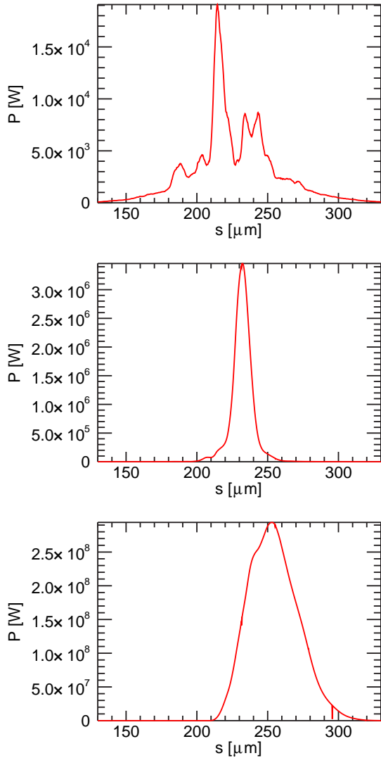
Figure 6: Detuned cavity length: From top to bottom are shown Genesis 1.3 simulations of pulse profiles after 1 pass, 3 passes and at saturation (after 8 passes).
