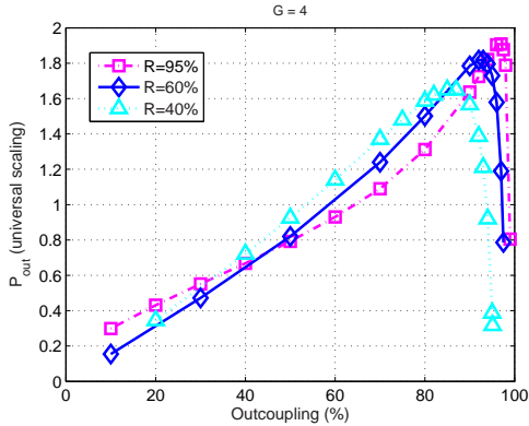
Figure 4: Output power as a function of outcoupling fraction, for different mirror reflectivities and G = 4 . The curve for 60% reflectivity is in blue.
