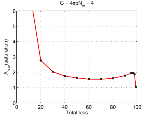
Figure 2: Intracavity saturation intensity as a function of total cavity loss, for a gain parameter G = 4\pi\rho N_w = 4 . The data is from 1D steady state oscillator simulations.
