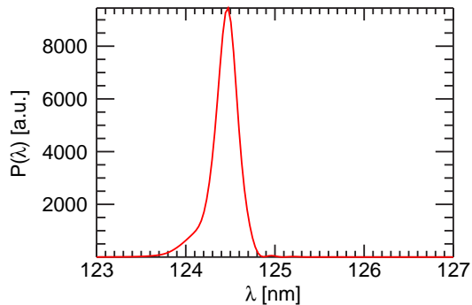
Figure 7: Detuned cavity length: Genesis 1.3 simulation radiation spectrum at saturation (after 8 passes).
